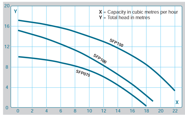
Performance Curve
