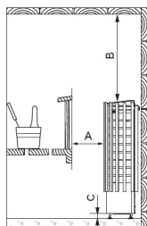
Safety distances (all dimensions in millimeters)
