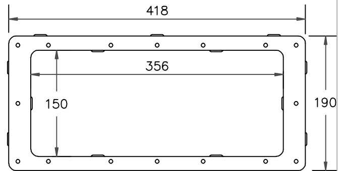
LINER PLATE ADAPTOR (PT NO. HD101-3)
